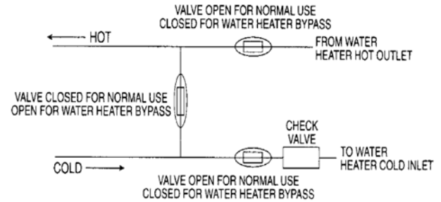
Typical Water Heater Bypass Valve diagram
