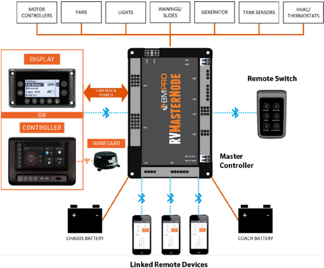
This illustration shows a typical Rapid Camp+ system layout. The Touchscreen Control Panel is Bluetooth linked to the Master Node, which in-turn controls the electrical devices of the motorhome.
