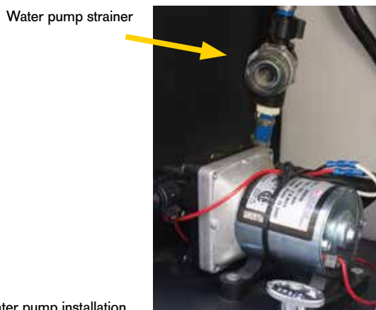
Typical water pump installation
