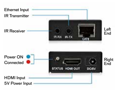
Typical Receiver Input/Output Ports
